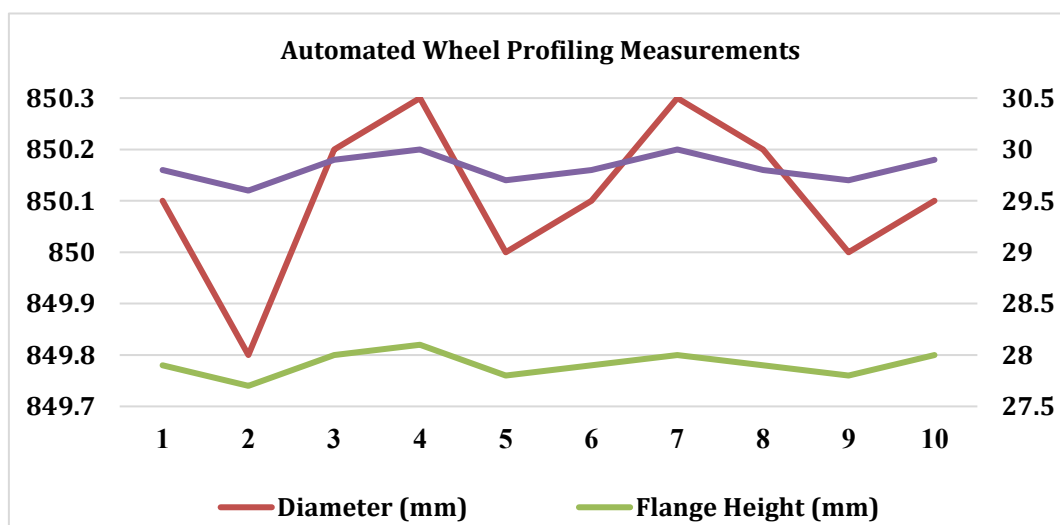
Fig. 8. Automated wheel profiling measurements
