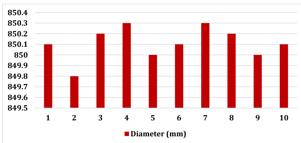
Fig. 5. Automated diameter measurements
